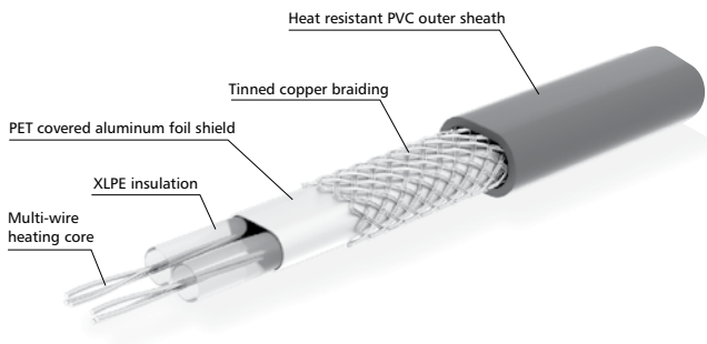
ELEKTRA SnowTec® heating mat's cable structure
